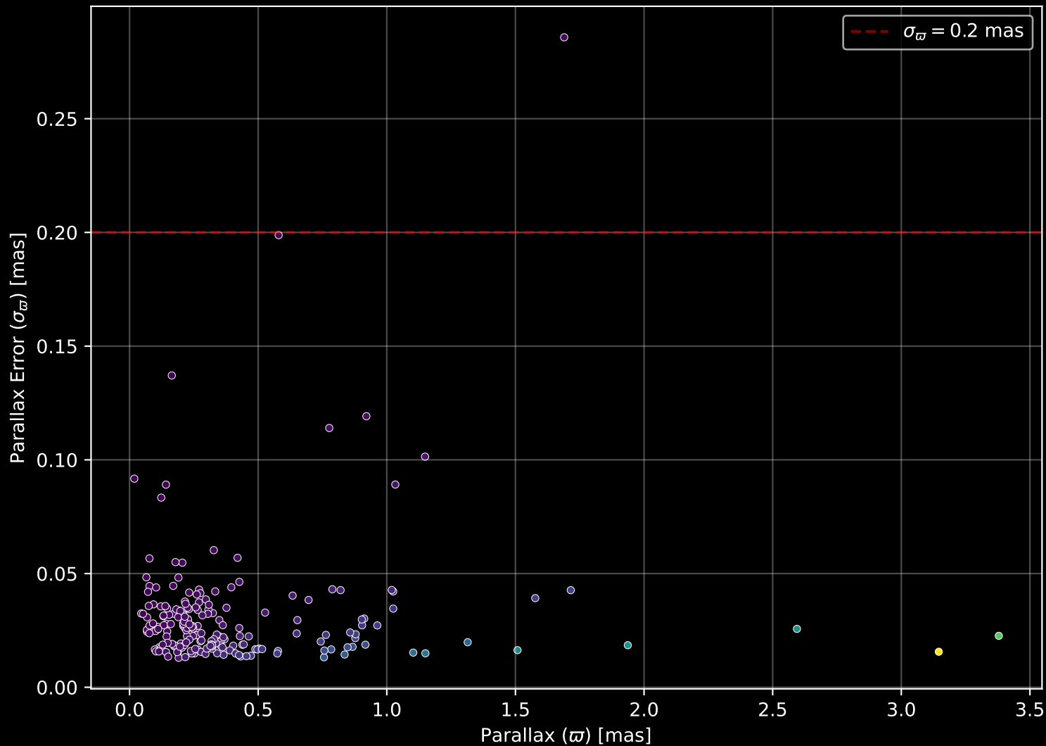
APOGEE DR17 Field: [225+00] Parallax Quality (n= 200)
