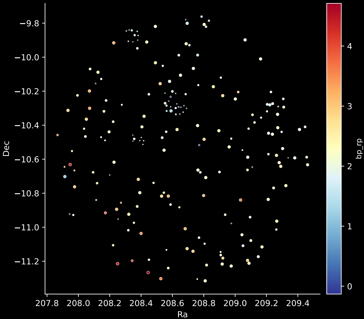
APOGEE DR17 Field: [225+00] Stars: 200
