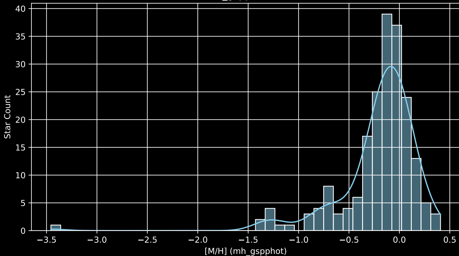
APOGEE DR17 Field: [225+00 [M/H] (mh_gspphot) (n= 200)
