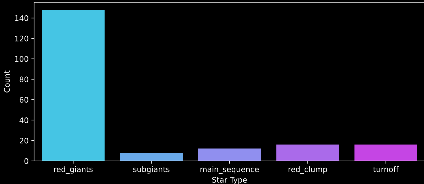
APOGEE DR17 Field: [225+00] Count plot of Star Type
