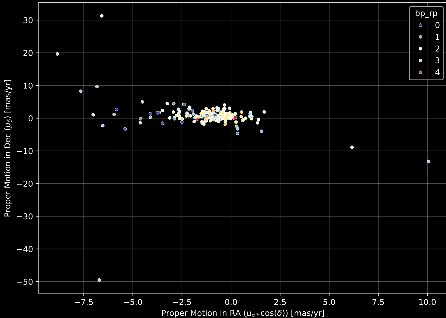
APOGEE DR17 Field: [225+00] Proper Motion Diagram (n= 200)
