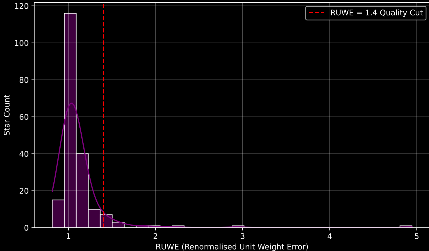
GAPOGEE DR17 Field [225+00] RUWE Distribution (n= 196)
